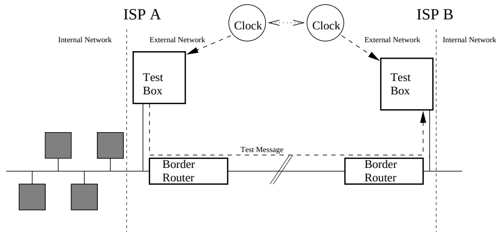
Figure 2: Experimental Setup
